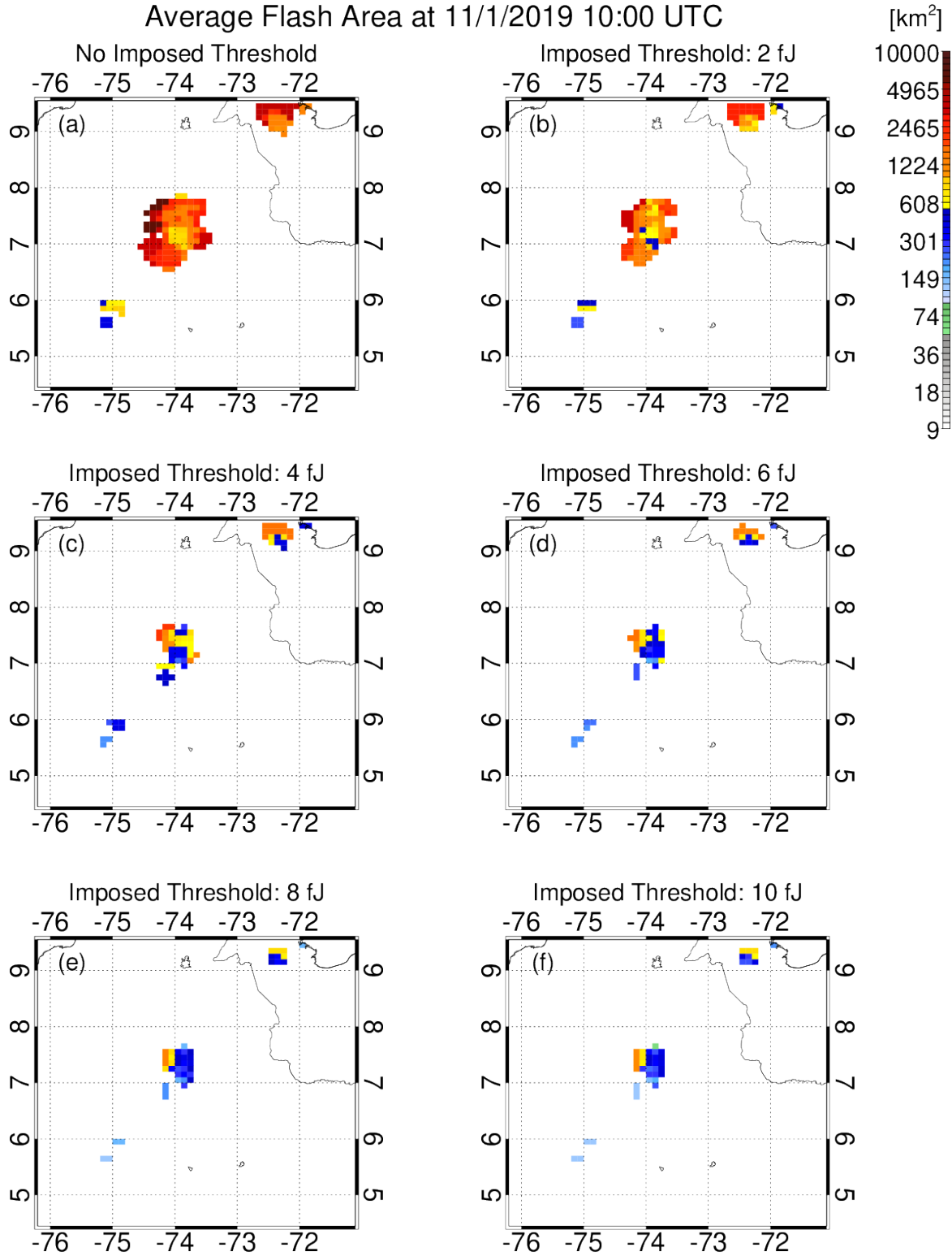
Figure 8. Average Flash Area (AFA) grids generated from (a) the original GLM data and the reclustered data under artificial thresholds of (b) 2 fJ, (c) 4 fJ, (d) 6 fJ, (e) 8 fJ, and (f) 10 fJ.
