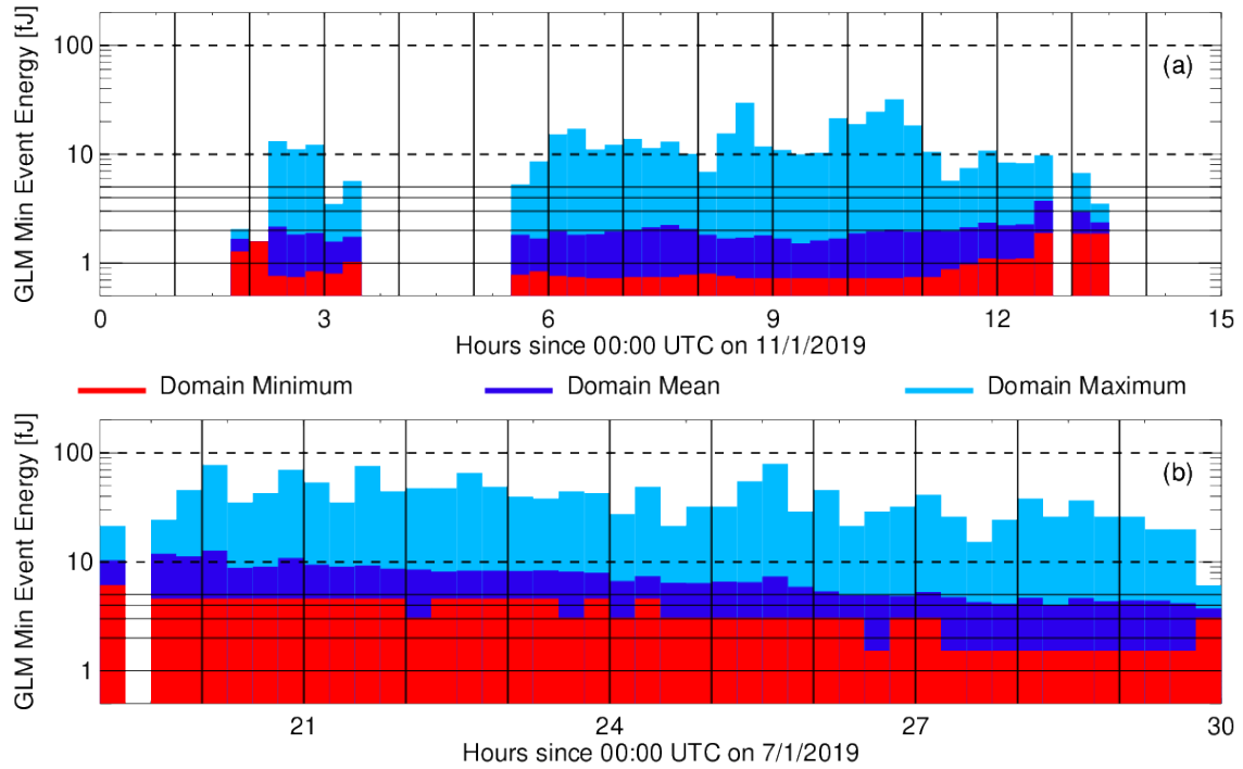
Figure 1. Timeseries of GLM minimum event energy during a thunderstorm over (a) Colombia near the satellite subpoint where thresholds are generally low and (b) Colorado where thresholds are known to be relatively high. Minimum event energies are computed for every pixel and the minimum (red), mean (dark blue) and maximum (light blue) values over each region are reported.
