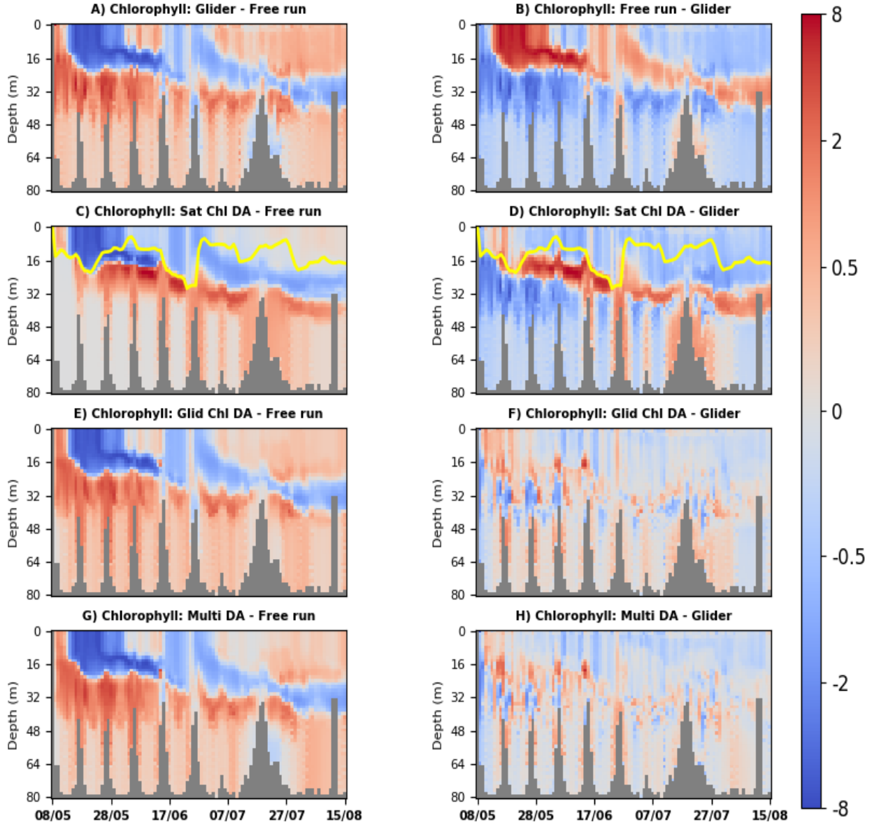
Figure 5. The left hand panels (A,C,E,G) demonstrate the spatio-temporal impact of the multi-platform system components on the simulated chlorophyll a concentrations (mg m -3 ) by comparing different simulations to the free run. One major advantage of the left-hand side panels is that they demonstrate how the changes introduced by the assimilation propagate vertically with the model dynamics, e.g. for the satellite OC assimilation (panel C) that updates the model only in the mixed layer (the MLD is marked in panels C-D by a yellow line). The right hand panels (B,D,F,H) show the skill of each component by comparing the simulations to the glider observations. The first row shows the skill of the free run (panel B) and the required changes to the free run in order to better match the glider observations (panel A). The rows beneath the first row compare the chosen reference (free run or glider) with a range of system components: i) the reanalysis assimilating satellite OC chlorophyll (panels C and D), ii) the reanalysis assimilating glider chlorophyll (panels E and F) and iii) the multi-platform assimilation (joint physical data, glider chlorophyll and oxygen, and satellite chlorophyll assimilation, panels G and H).
