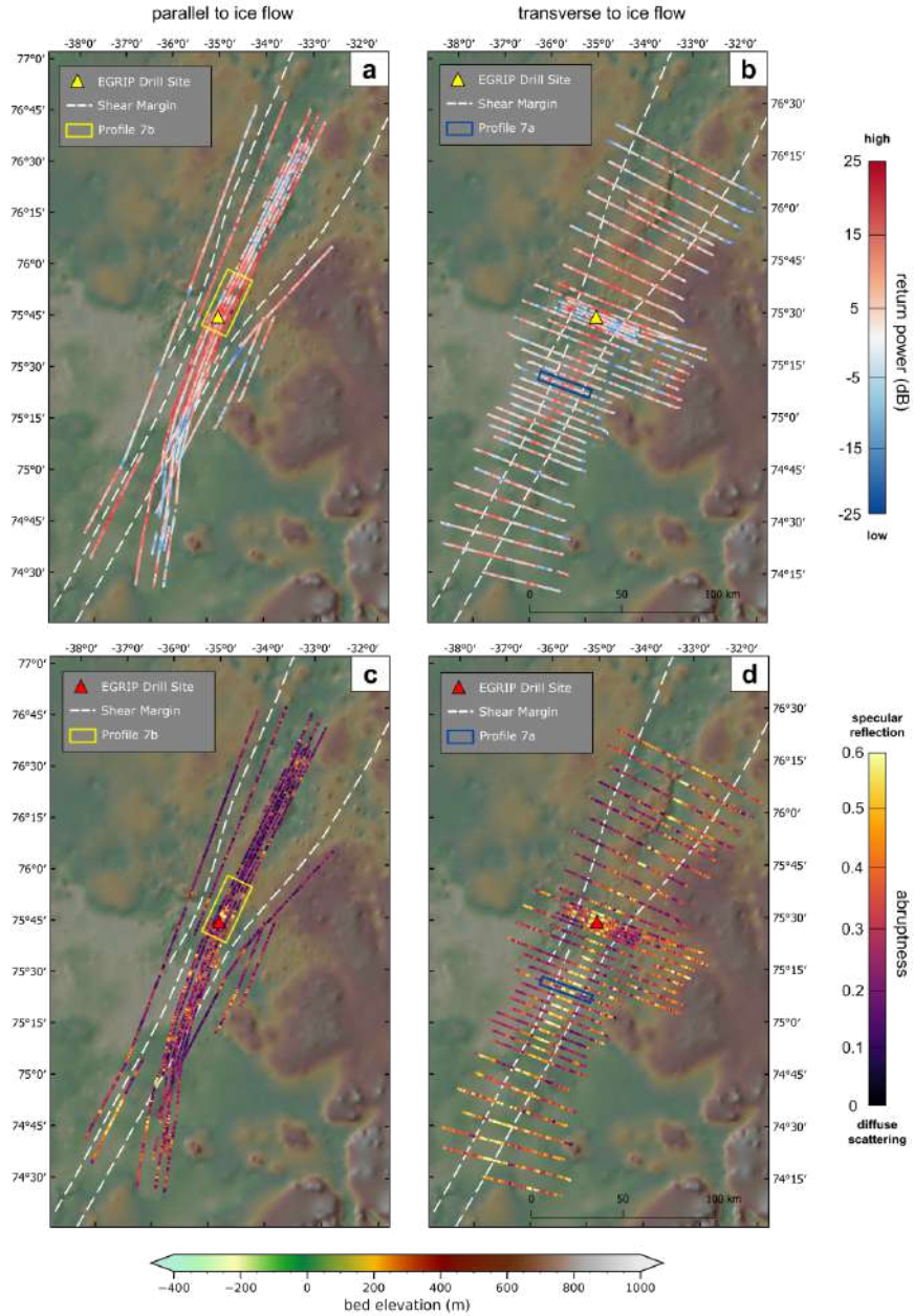
Figure 6: Bed echo characteristics for (a and b) basal return power and (c and d) waveform abruptness for profiles oriented along-flow (a and c) and across-flow (b and d), respectively. Basal return power is corrected for spherical spreading as well as englacial attenuation losses (8 dB/km ice thickness) and displayed in decibel (dB with respect to unity). Waveform abruptness is expressed as the ratio between the maximum BRP and the integrated bed return power and is thus unitless. High values (yellow) represent the dominance of specular reflection and low values (dark purple) the dominance of diffuse scattering of the base. The yellow and blue rectangular outlines indicate the position of the radargrams in Figure 7. The interpretation of bed permittivity from the BRP data presented here is limited due to the simple correction scheme for englacial attenuation applied here. A large part of the spatial heterogeneity in BRP probably results due to an inaccurate englacial attenuation correction, which cannot be overcome due to an uncertainty in englacial temperature distribution.
