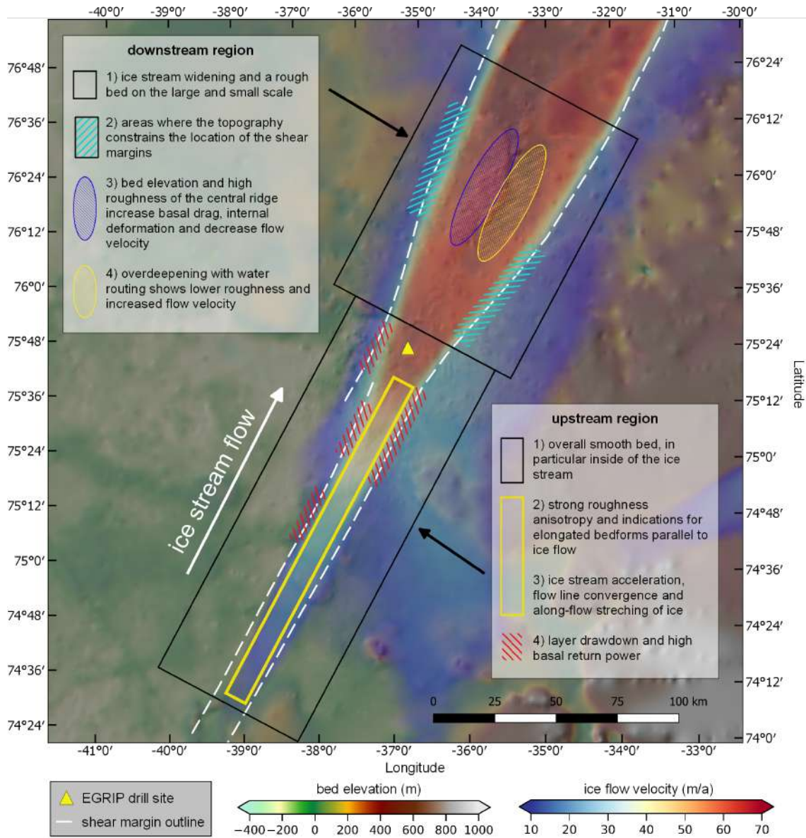
Figure 10: Summary of the basal properties of the (a) upstream and the (b) downstream survey region.
