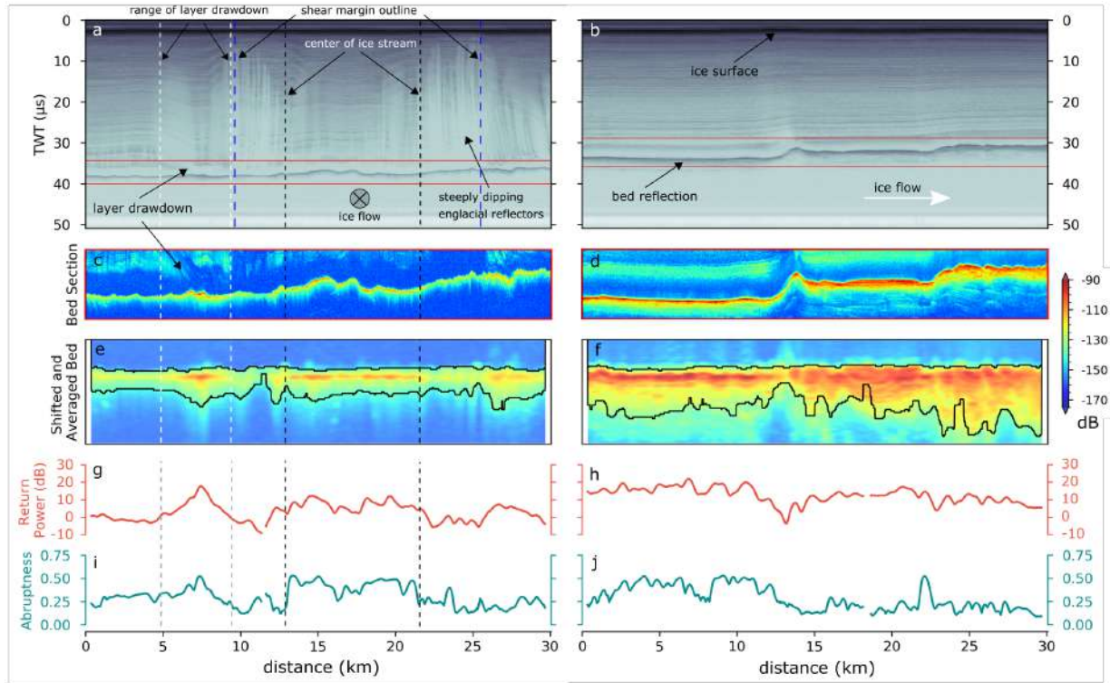
Figure 7: Two radar sections (two-way travel time (TWT) on the y-axis) and basal return echo properties from (a) an across-flow profile (location is indicated in Figure 6b and d with the blue outline) and (b) an along-flow profile (location is indicated in Figure 6a and c with the yellow outline). Panels c and d represent the analysis window of the ice-bed interface of the corresponding radargrams (indicated with the red lines in the radargrams) and their amplitude in dB. Panels e and f show the elevation-levelled basal reflectors and the corresponding BRP after along-track averaging. The black outline represents the window of integration for basal return power. The radargrams in panels a-f are neither corrected for spherical spreading nor englacial attenuation. Panels g and h show BRP corrected for spherical spreading as well as englacial attenuation (8 dB per km ice thickness) and (i and j) the waveform abruptness. The blue dashed lines in (a) show the position of the shear margins, the white dashed lines the region of layer drawdown outside of the shear margins and the black dashed lines the central part of the ice stream.
