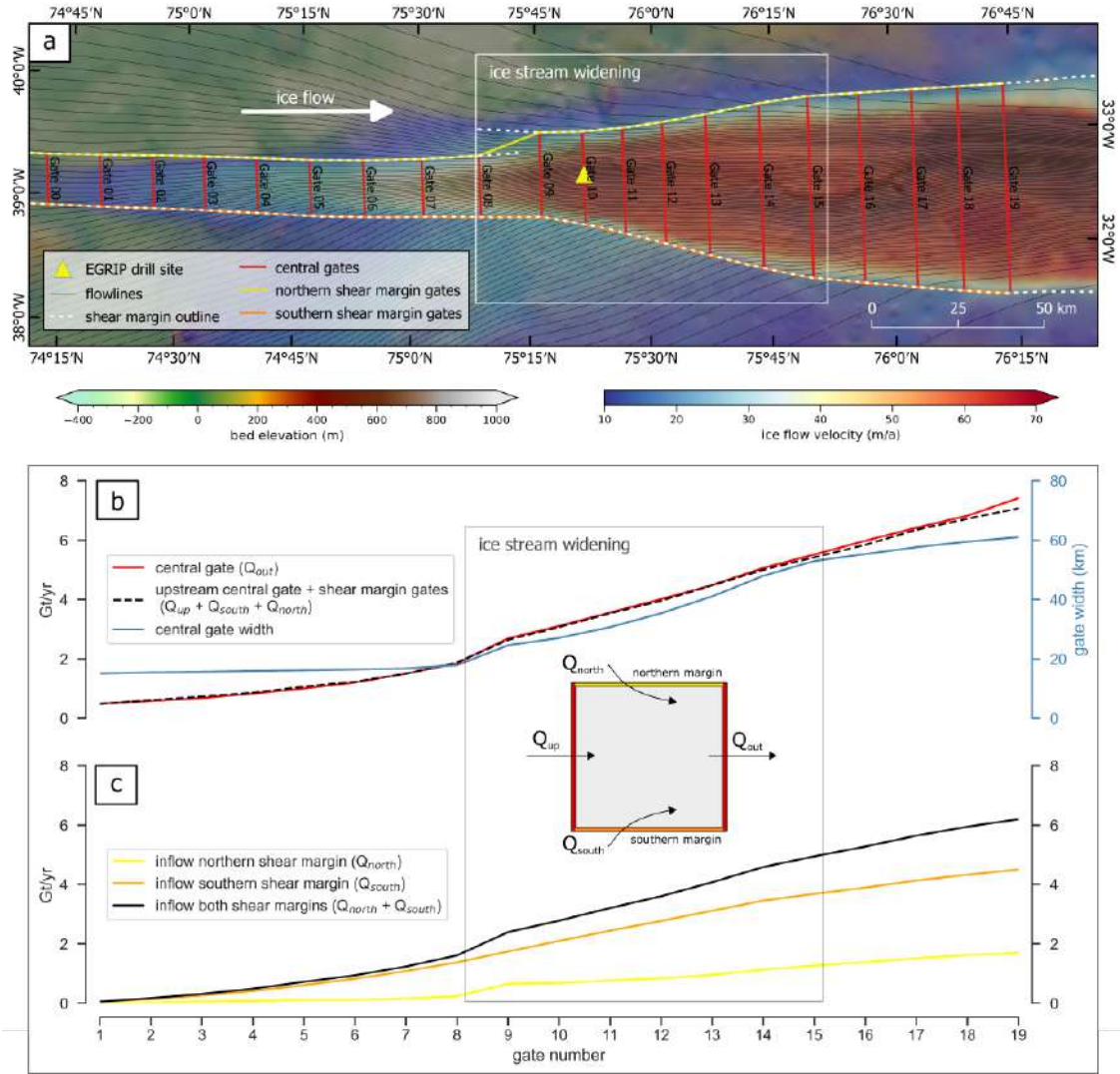
Figure 3: Flux gate analysis of the onset of the NEGIS. Panel (a) shows the position of central flux gates (red) and flux gates at the shear margins (yellow and orange, respectively). The location where the ice stream widens is marked with a white outline. Panel (b) shows the mass flux (in Gt/yr) through the central gates ( Q_{out} ; red line) in comparison to the sum of the respective upstream central gate ( Q_{up} ) and the corresponding shear margin gates ( Q_{south} + Q_{north} ; black dashed line). The blue line represents the width of the central gates. The cumulative mass flux through the northern and southern shear margin (as well as the sum of both) is shown in panel (c).
