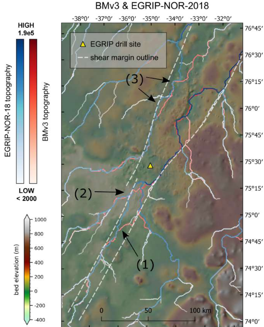
Figure 8: Basal water routing pathways calculated based on EGRIP-NOR-2018 bed elevation (Franke et al. (2020b); in blue) as well as pathways calculated with the bed elevation model BMv3 (Morlighem et al. (2017); in red). The basal water routing colour saturation represents the number of accumulated upstream cells. Pixels containing less than 2000 upstream cells are transparent. High values and dark colours represent pathways that transport larger amounts of upstream cells. Features (1) – (3) present locations where the routing pathways from the two bed elevation models show the largest deviations. The background map represents the bed elevation of the EGRIP-NOR-18 data.
