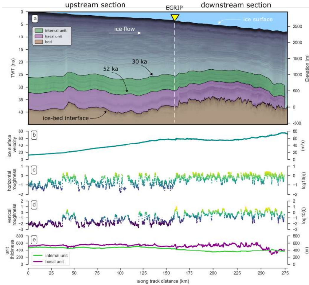
Figure 4: Evolution of several basal and englacial properties in ice flow direction, extending from far upstream to the downstream end of our survey area (red line in Figure 1 and 5). Because there is no continuous survey profile, the downstream part (right part of the dashed line) is offset \sim 1 km to the South-East (transverse to along-flow profile orientation) relative to the upstream profile (left of the dashed line). The transition between the two profiles marks the position of the EGRIP drill site (yellow triangle). Ice flow direction is from left to right. (a) along-flow radargrams with continuously tracked surface (white), two internal ice units (basal unit in purple and internal unit in green) and bed reflection (red dashed line); (b) ice surface flow velocity; (c) horizontal roughness \eta and (d) vertical roughness \xi , both with the same colour code and scaling as in Figure 2; and (e) the thickness of the internal and basal unit.
