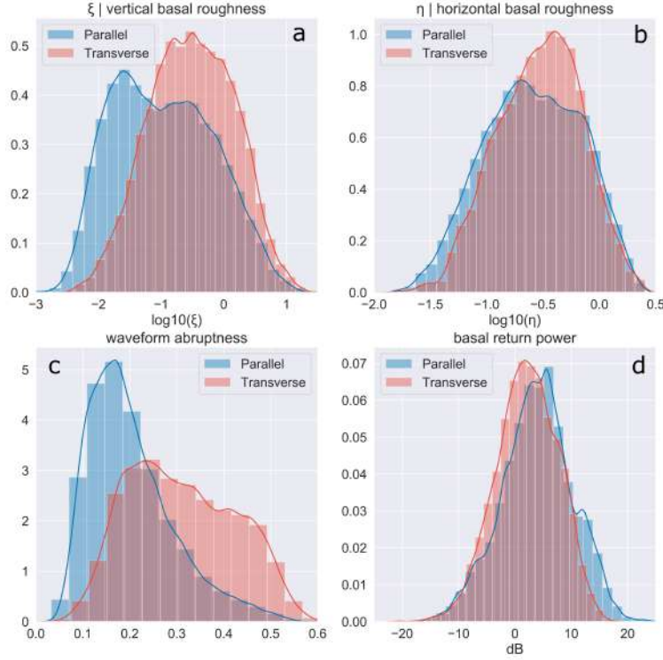
Figure 9: Histograms presenting the distribution of (a) vertical basal roughness, (b) horizontal basal roughness, (c) waveform abruptness and (d) BRP for profiles oriented along- and across-flow for the location inside of the ice stream. The interpretation of anisotropy of BRP is limited due to the simple correction scheme for englacial attenuation. Blue bins represent along- and red bins across-flow profiles. The y-axis shows the kernel density estimation.
