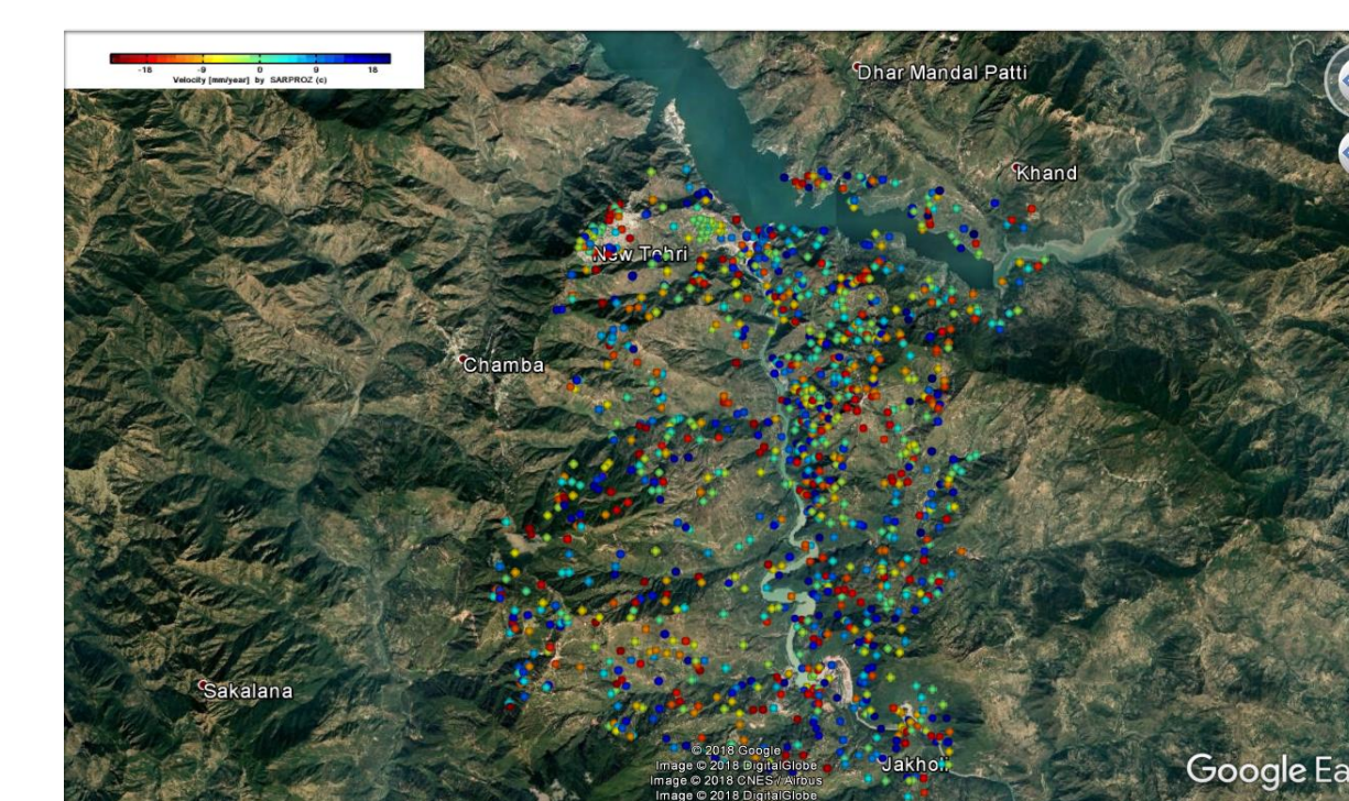
Figure 7. Time-Series Displacement of PS depicted on Google Earth
