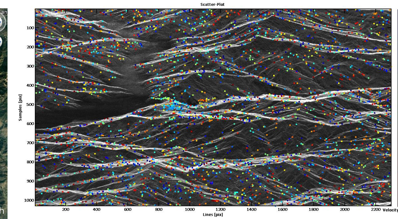
Figure 8. LoS velocity of PS in SAR coordinate system. Dark feature is the reservoir.
